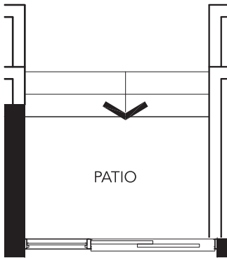
+Patio @ Ground Floor 51 sq.ft. - Suite - 04/06
