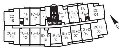
M2 - Typical Floor Plan 4th-15th Floor
